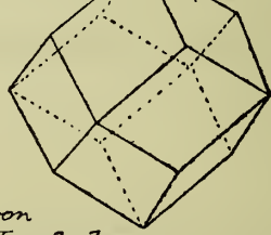
Irregular rhombic dodecahedron
